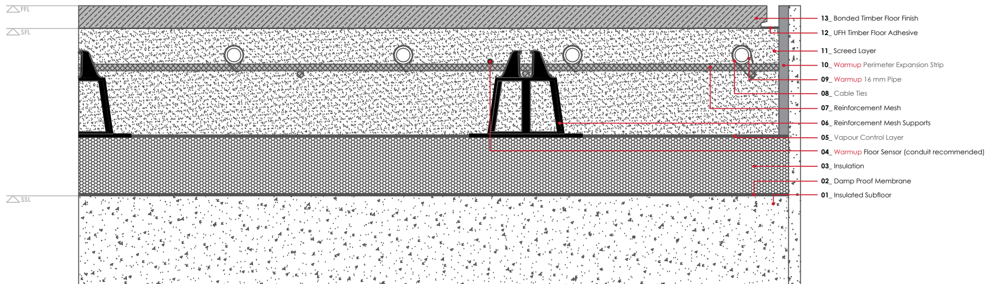
WARMUP FORTE SYSTEM. Bonded Timber Floor Finish
