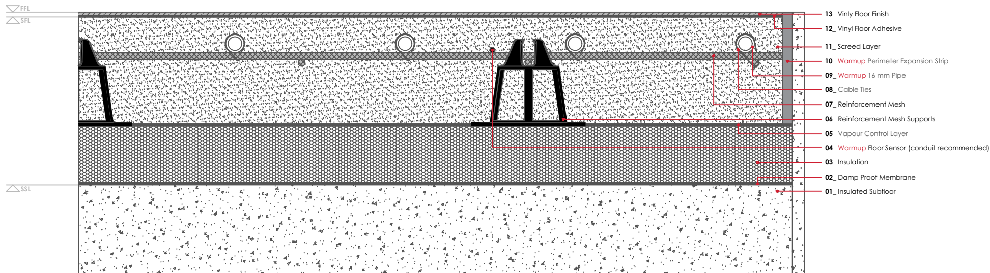
WARMUP FORTE SYSTEM. Vinyl Floor Finish - Glued
