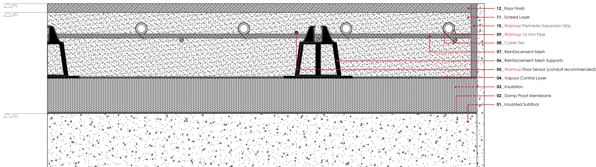
WARMUP FORTE SYSTEM. Standard Detail
