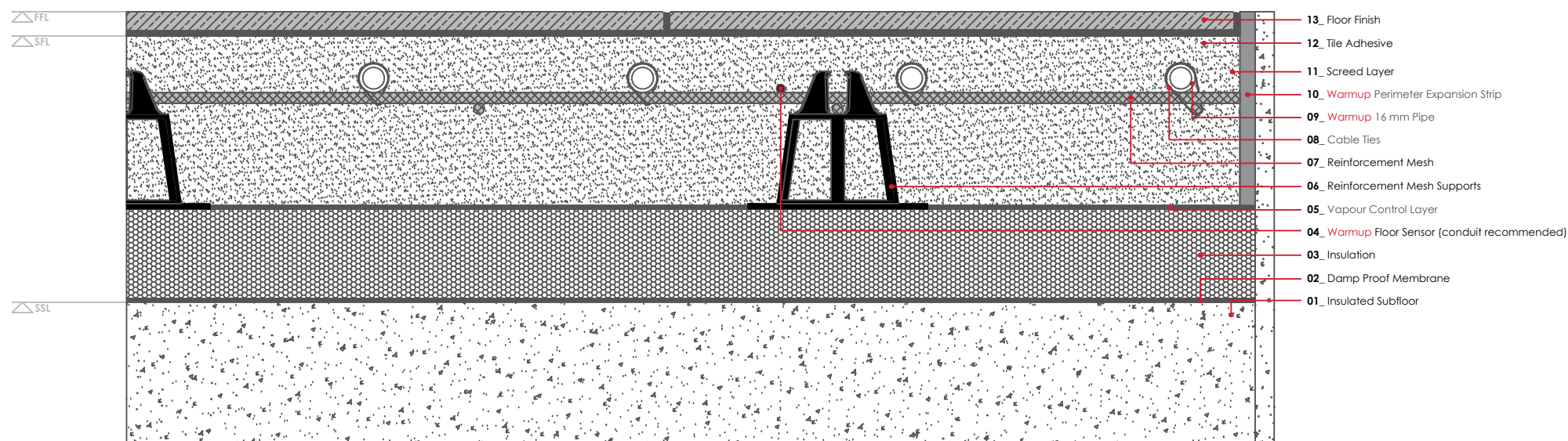
WARMUP FORTE SYSTEM. Tiled Floor Finish
