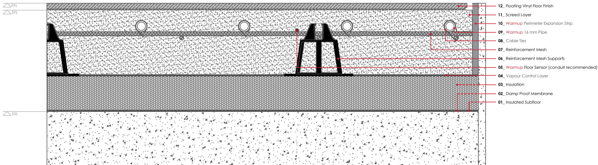
WARMUP FORTE SYSTEM. Vinyl Floor Finish - Floating
