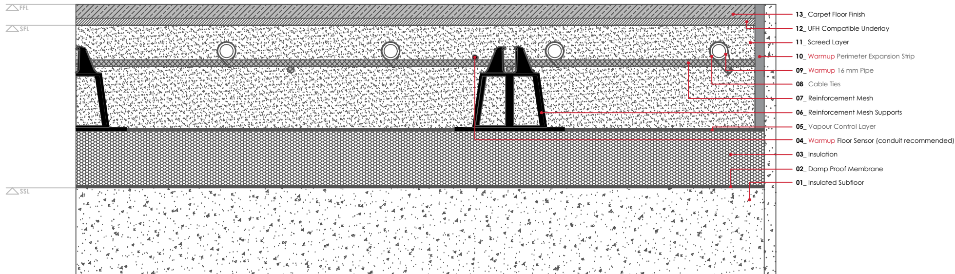
WARMUP FORTE SYSTEM. Carpet Floor Finish
