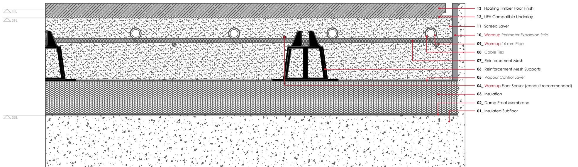
WARMUP FORTE SYSTEM. Floating Timber Floor Finish
